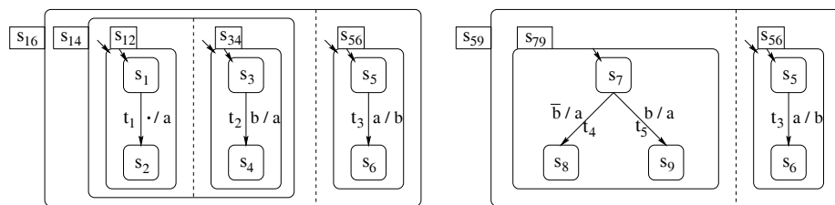
Fig. 1. Two example Statecharts
