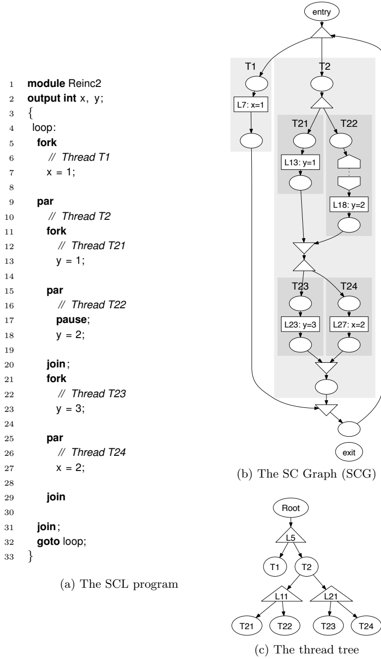
Figure 5: The Reinc2 example, a more elaborate example of thread concurrency and thread reincarnation
